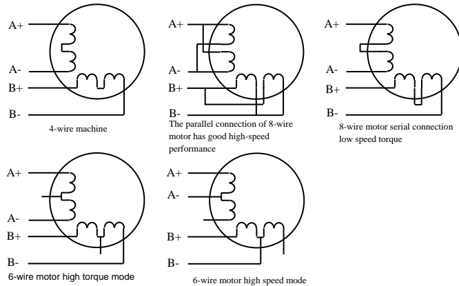
Figure 6 Motor Wiring
