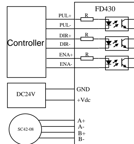
Figure 7 Typical Connection
