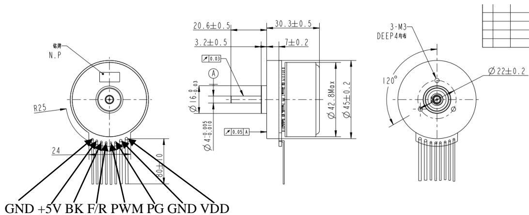
FIG. 1 Mechanical dimensions
